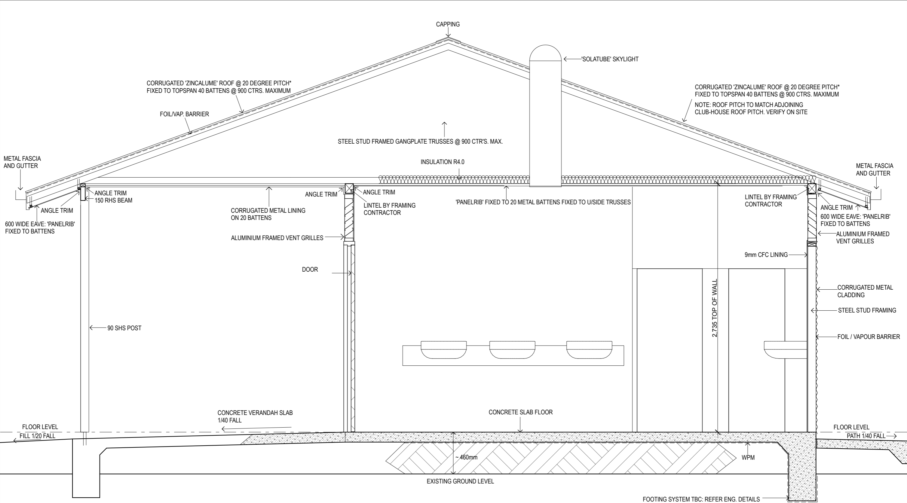
SECTION A - A 1:25 SCALE
